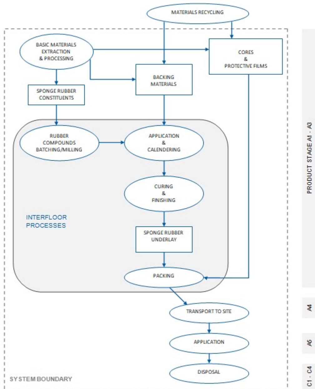
INTERFLOOR'S WAFFLE FOAM UNDERLAY LIFE CYCLE
